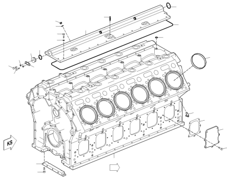
CRANKCASE UPC.06A01 2080
